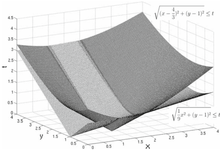
Fig. 2 Nonlinear conic mixed-integer rounding cut
