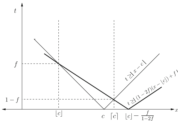
Fig. 1 Simple conic mixed-integer rounding cut
