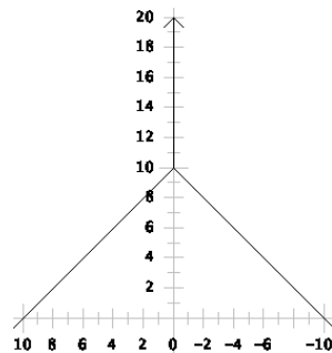
FIGURE 16. The thermograph of the switch \{10 | -10\} .
