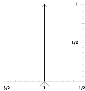
FIGURE 15. The thermograph of the tepid game \{1 | 1\} = 1^* .
