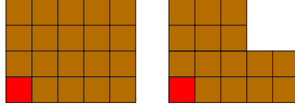
FIGURE 18. Two CHOMP positions. The red piece in the lower left is poisoned and cannot be eaten. The first player pointed at (3, 2) and chomped off four pieces.
