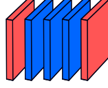
FIGURE 9. G_3 = \uparrow_1
