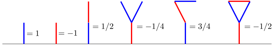
FIGURE 4. Some HACKENBUSH positions and their values.
