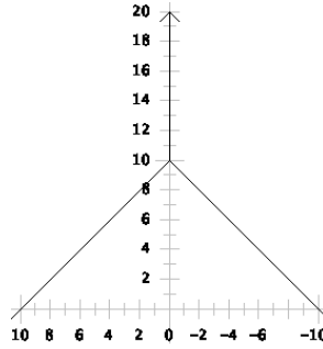
FIGURE 15. The thermograph of the switch \{10 \mid -10\} .
