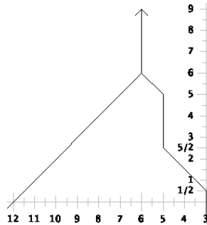
FIGURE 17. The thermograph of the game \{12 \mid \{5 \mid -5\}, \{3 \mid 2\}\} .
