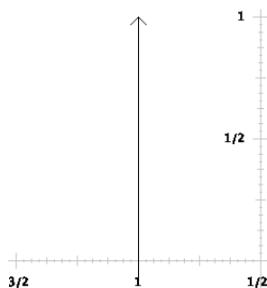
FIGURE 13. The thermograph of the number game 1.
