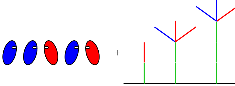
FIGURE 12. A BIPASS strip in disjunctive sum with a FLOWER GARDEN.
