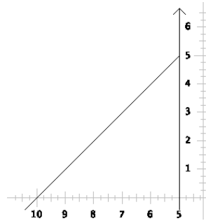
FIGURE 16. The thermograph of the game \{10 \mid \{5 \mid -5\}\} .
