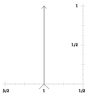
FIGURE 14. The thermograph of the tepid game \{1 \mid 1\} = 1^* .
