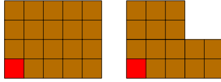
FIGURE 18. Two CHOMP positions. The red piece in the lower left is poisoned and cannot be eaten. The first player pointed at (3, 2) and chomped off four pieces.
