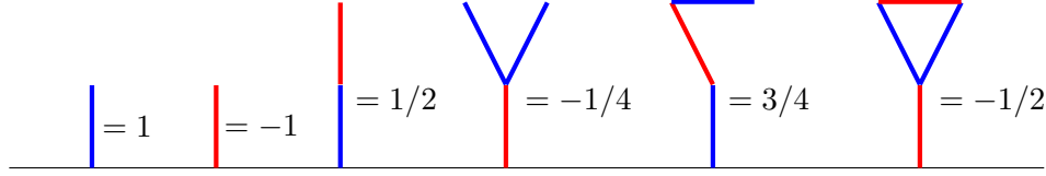
FIGURE 4. Some HACKENBUSH positions and their values.
