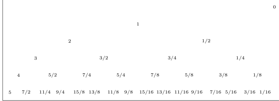
FIGURE 5. The births of the numbers in \mathbb{D} follow a binary tree structure. Each node has exactly two children. For example node 0 has the children -1 and 1 , and 3/4 has children 7/8 and 5/8 ; at the top, we find the birthday zero number, followed by the birthday one numbers, and so on. We display the nonegative number games born by day 5, and the negative ones are symmetrically obtained.
